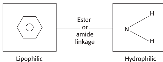
Fig. 6.6 Basic structure of local anaesthetics.
