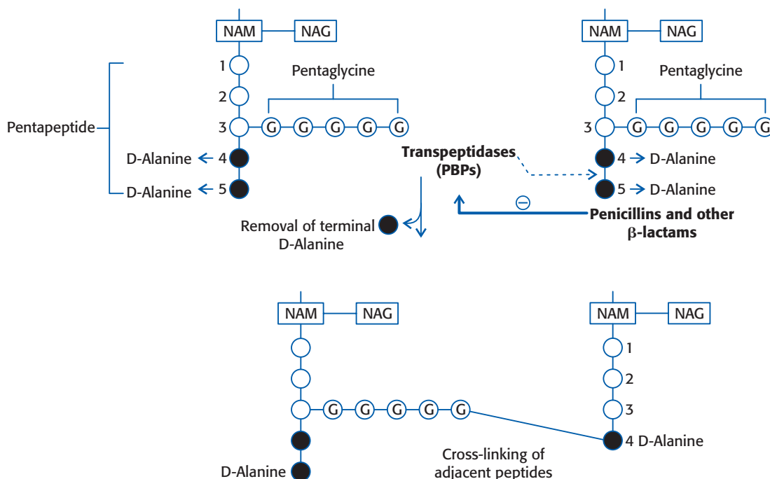
Fig. 11.6 Cross-linking of peptidoglycan residues and site of action of \beta -lactam antibiotics.
