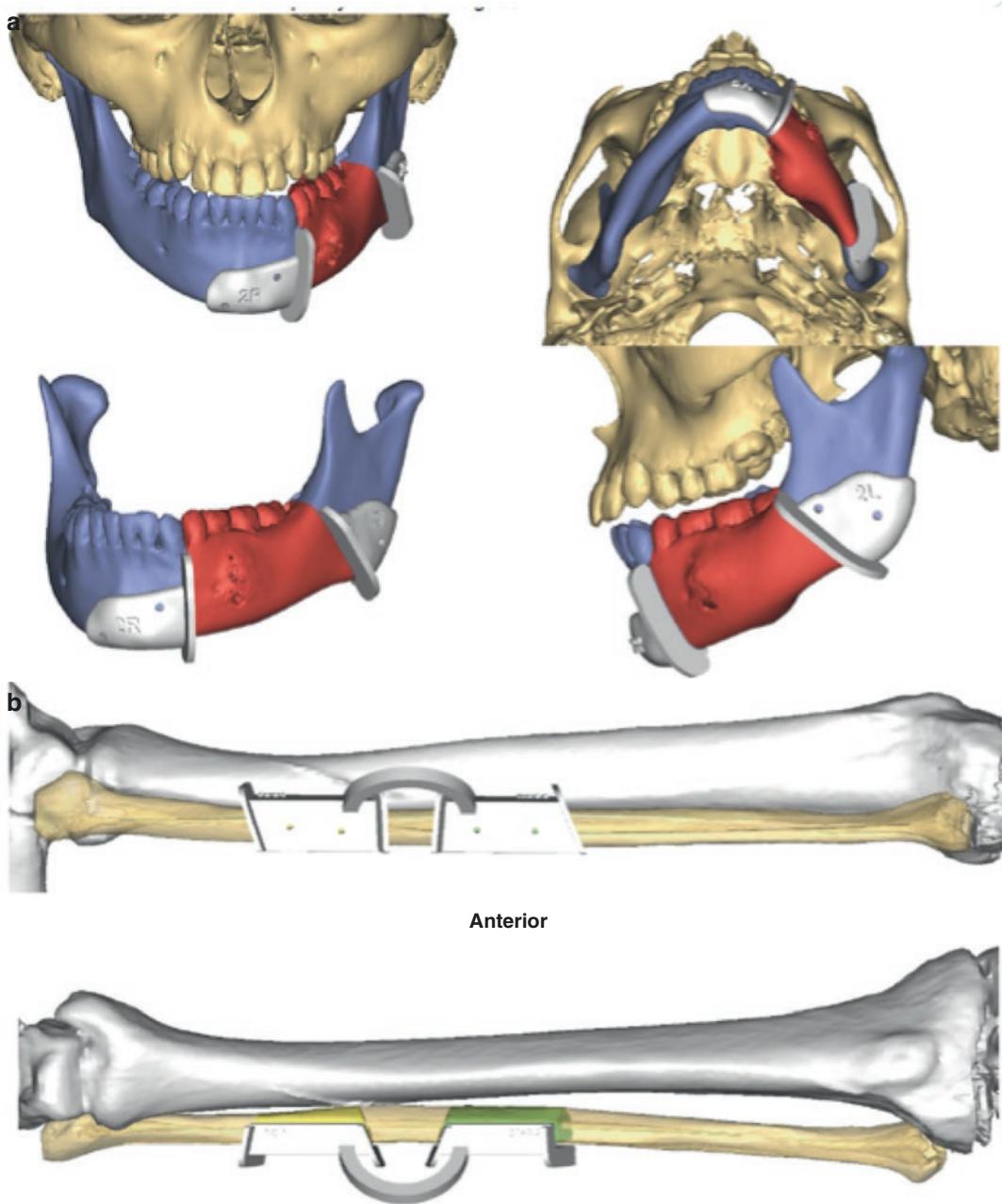
Fig. 13.9 (a) Ten-year-old patient with aggressive juvenile ossifying fibroma. Virtual design of the cutting guides to resect the tumor using Materialise® software. (b) Cutting guides for the fibula flap. (c) Design of the fibula flap placed with a “double barrel” technique for better esthetic
