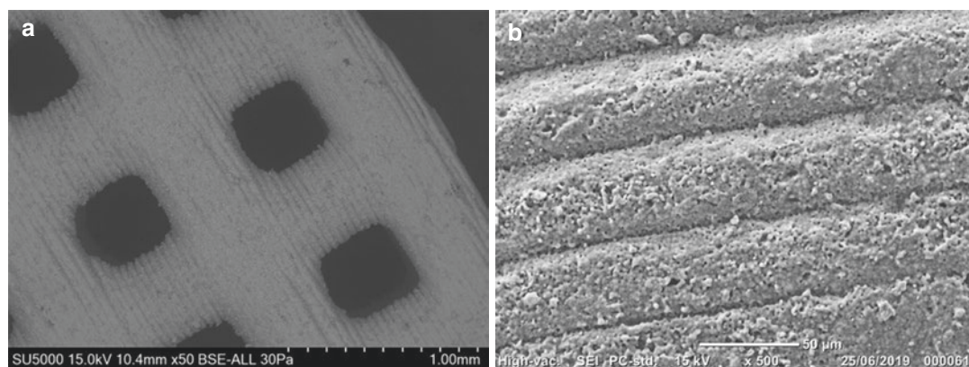
Fig. 2.2 (a) SEM morphology of BCP macroporous structure produced by ceramic stereolithography. (b) SEM morphology of \beta -TCP microporous structure produced layer by layer by ceramic stereolithography
